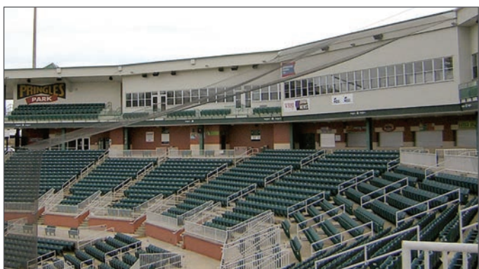
Cable Supported Backstop and Over-the-top Net System
